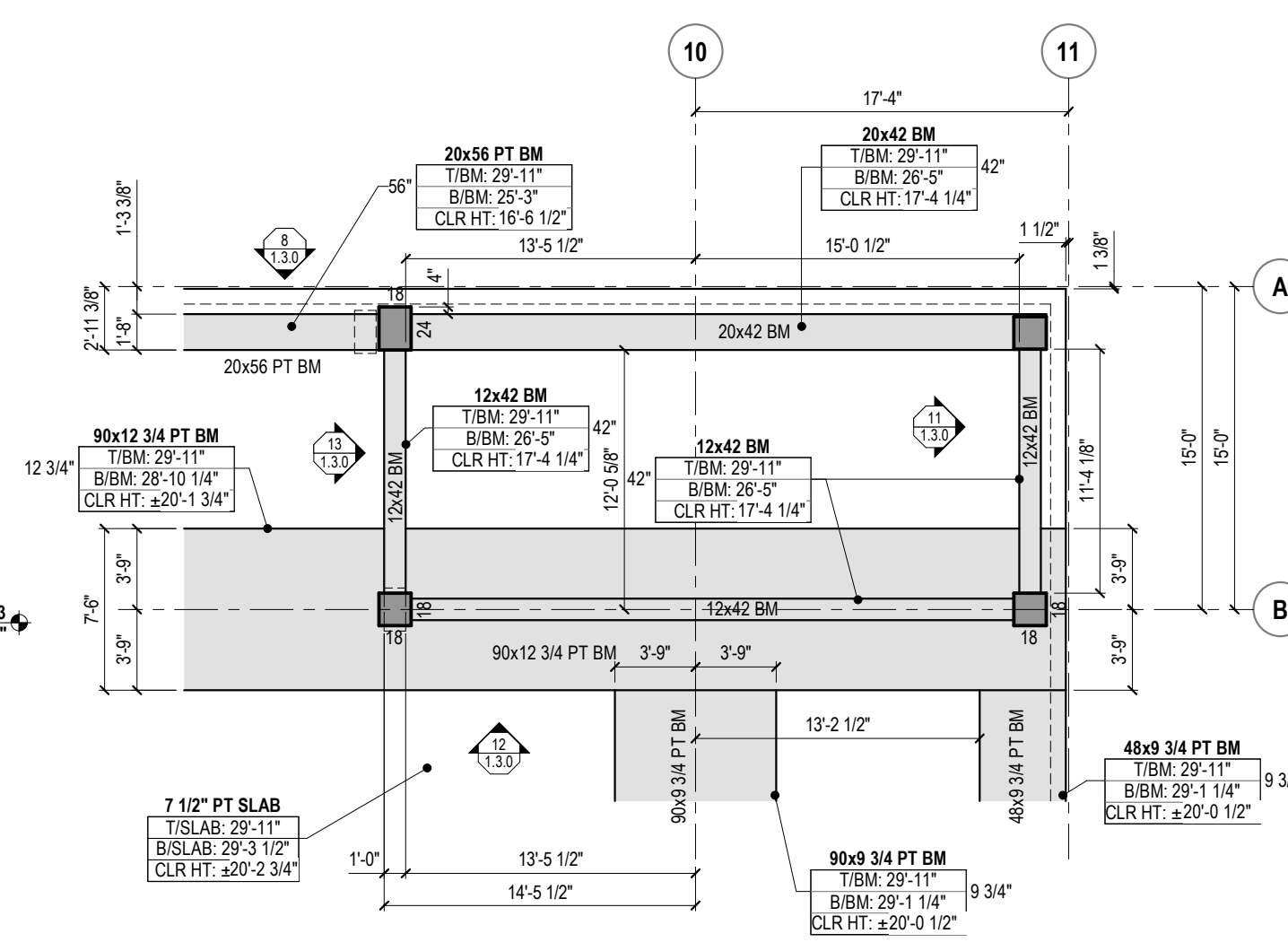
10 LEVEL 3 - NORTHEAST CALLOUT (SOFFIT PLAN) REF: 1/13.0
