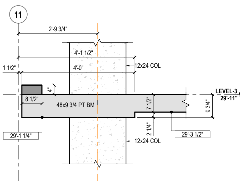
15 L3 - 48x9.75 BM @ GL 11
