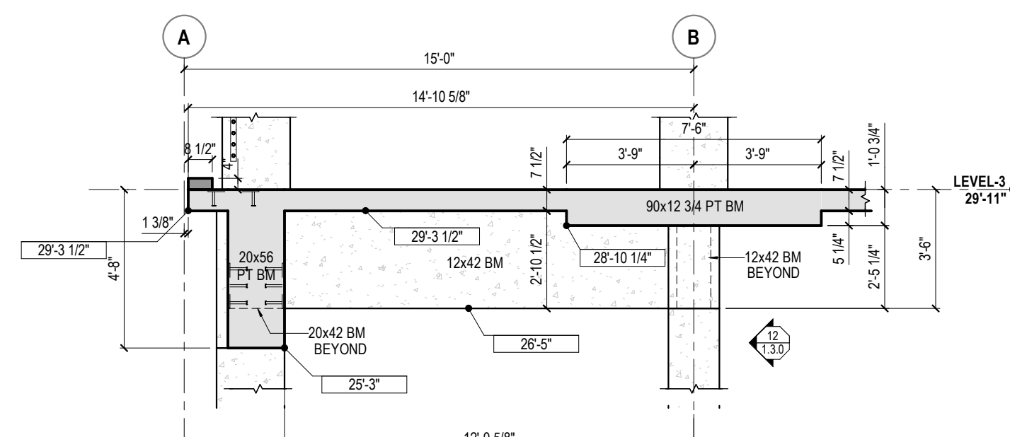
13 L3 - BEAMS @ GL (10,A-B)
