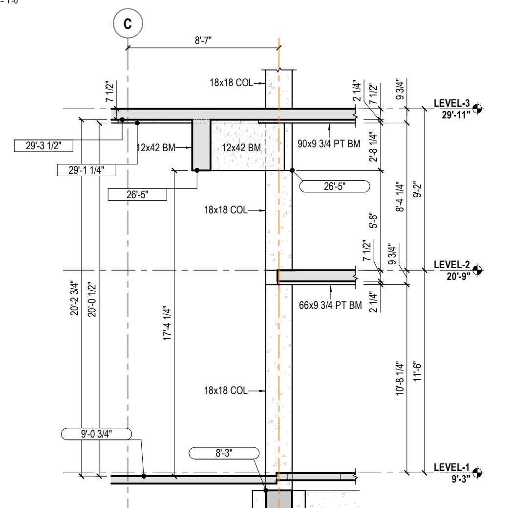
4 L3 - BUILDING ELEVATION @ GL (9-10,C)
