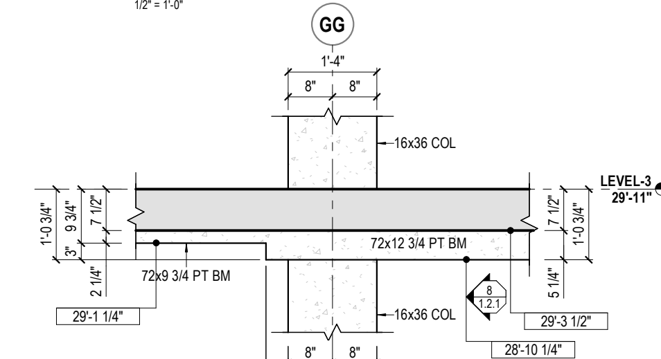
6 L3 - 3" SOFFIT TRANSITION @ GL (3,GG)
