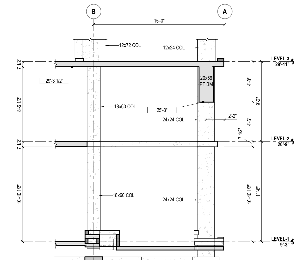
3 L3 - BUILDING ELEVATION @ GL (9,A-B)
