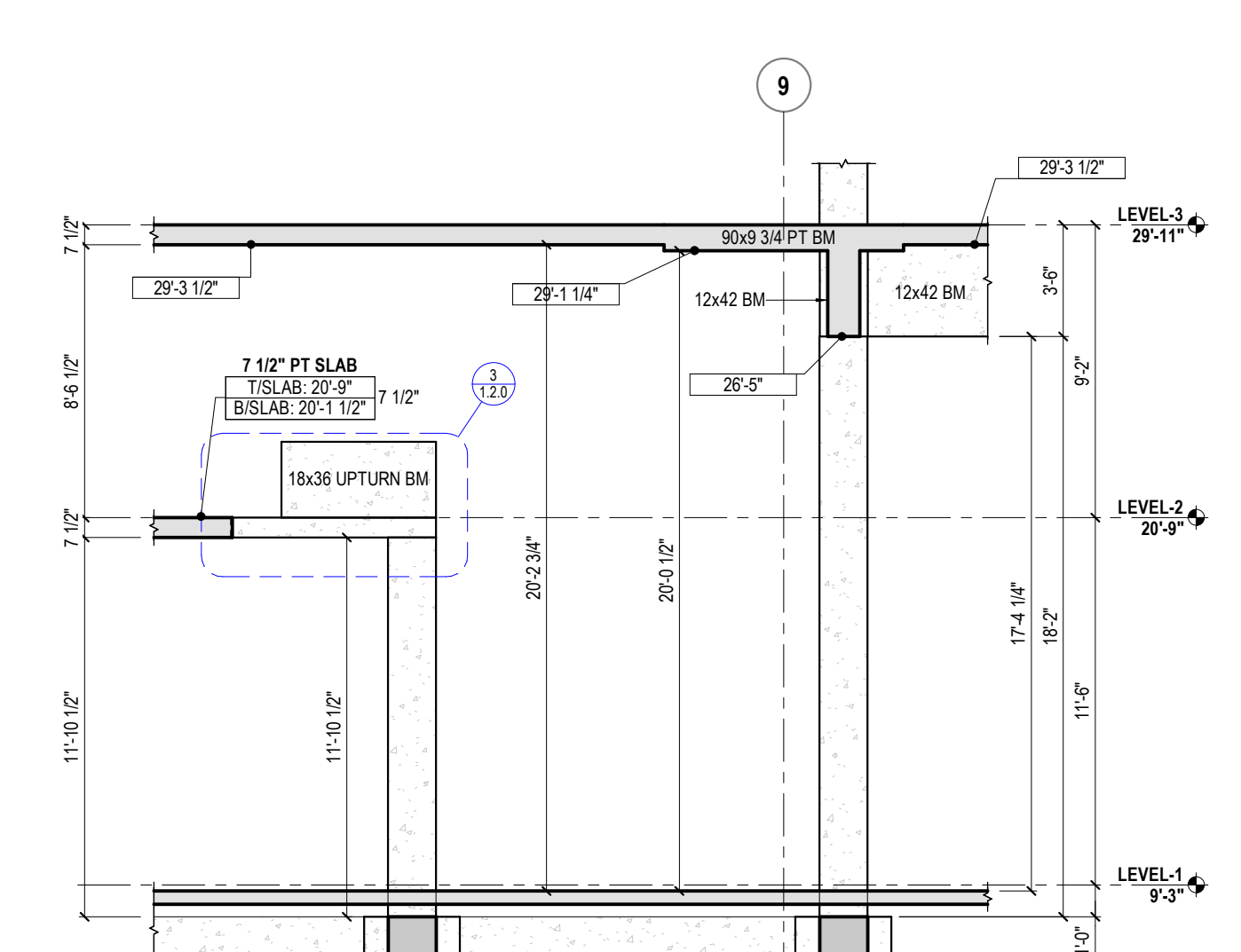
2 L3 - BUILDING ELEVATION @ GL (9,C)
