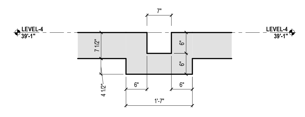
4 SECTION AT TRENCH DRAIN REF: 11.110
