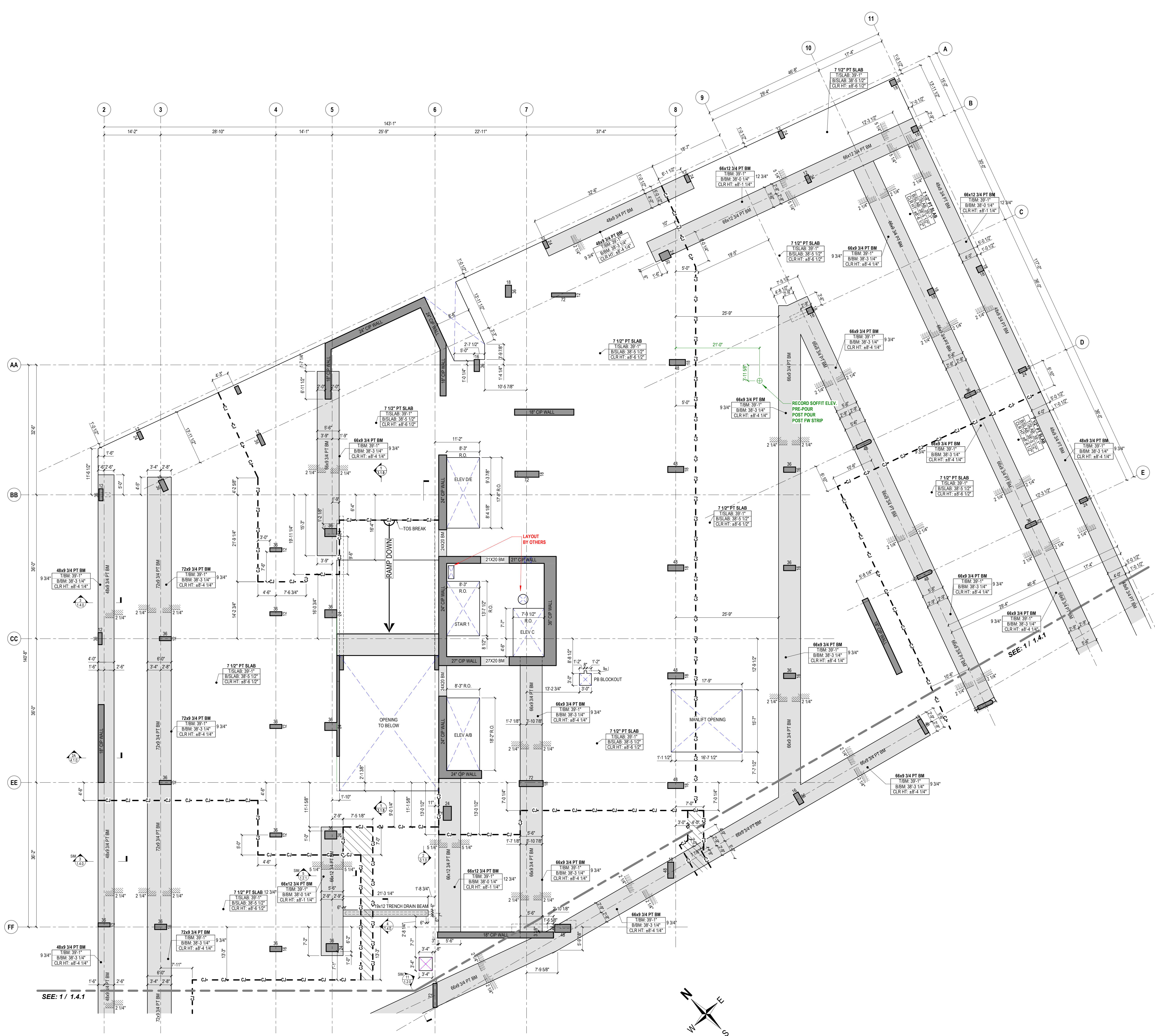
1 LEVEL 4 - NORTH AREA (SOFFIT PLAN) REF: 21.135
