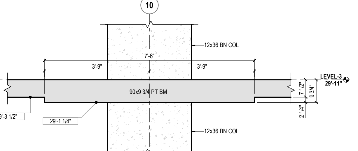
7 L3 - 90x9.75 BM @ GL 10
